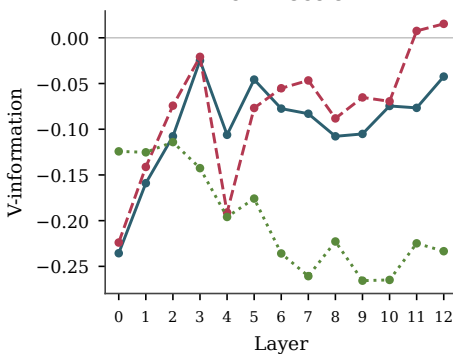
Arc Direction
