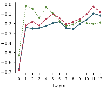
Phrase Role
