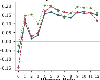
Phrase Role
