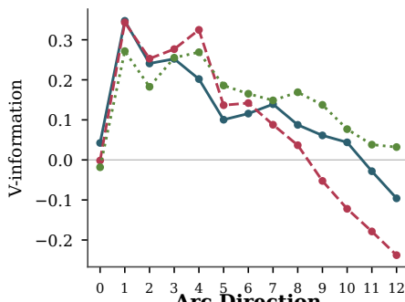
Arc Direction
